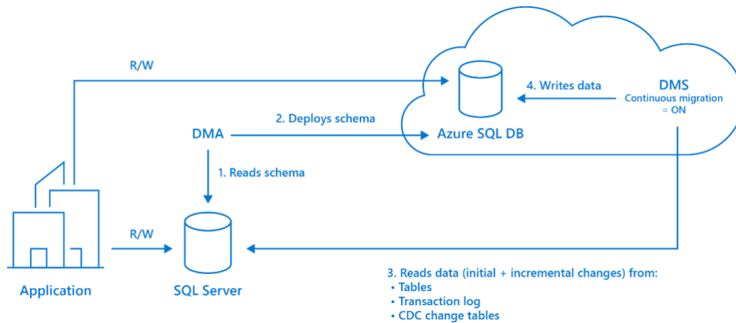
Figure 11 Continuous migrations workflow using DMA and DMS
